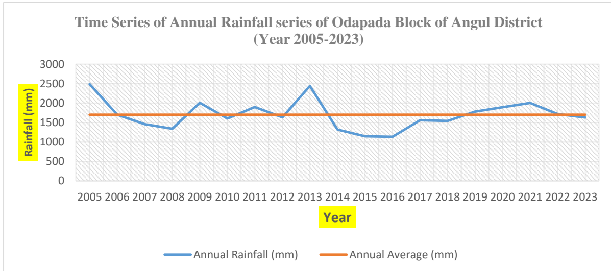
Fig.2.2 B. Time Series of Rainfall (Odapada Block)
