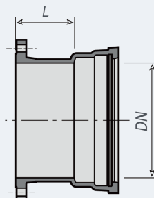
FLANGE - SOCKET
