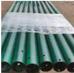
CHS- O/D- 76.1, T-3.6 MM
