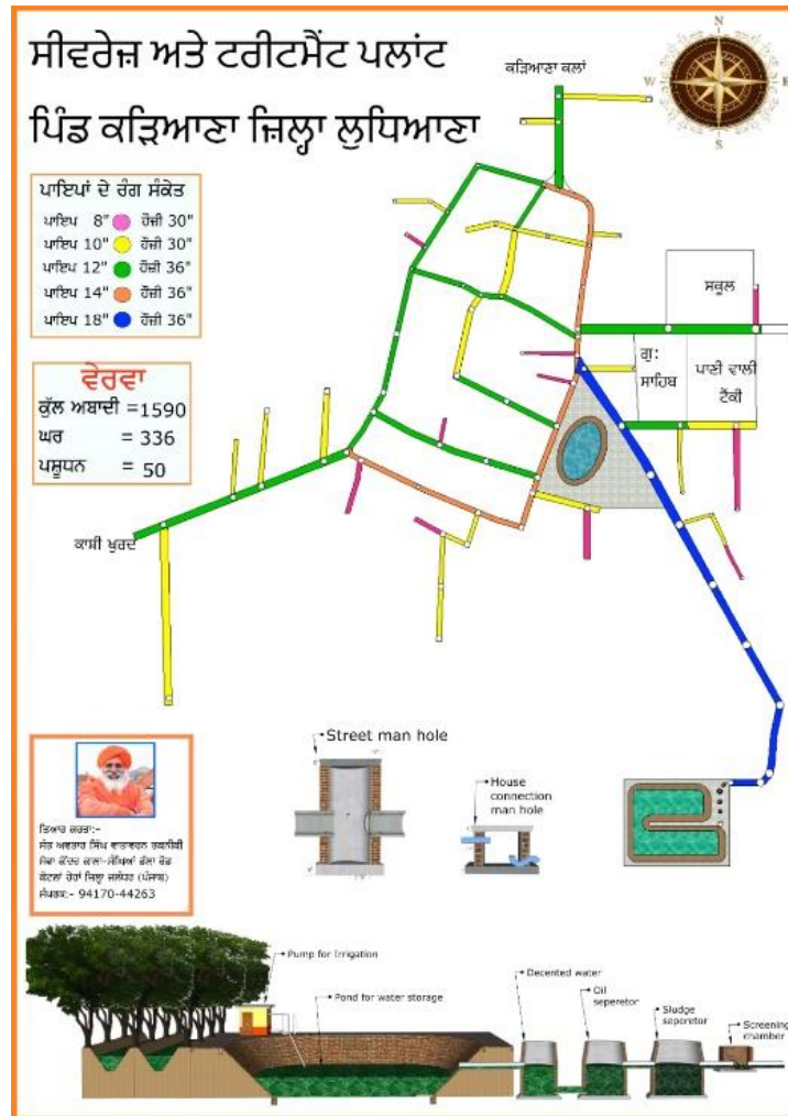
Layout of Seechewal Model to be executed in Kadiana Khurd
