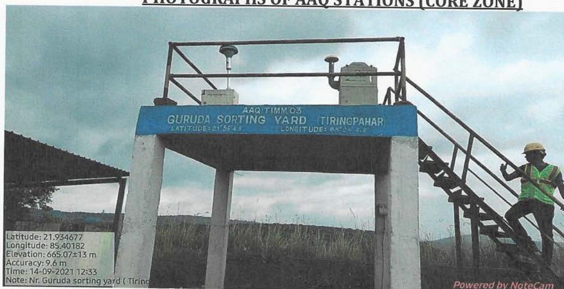
Fig.3 AAQ Station Near Guruda Sorting Yard (Tiringpahar Iron & Mn Mine)
